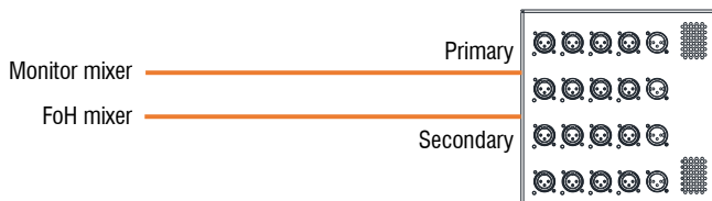
Switched mode (digital split example)
